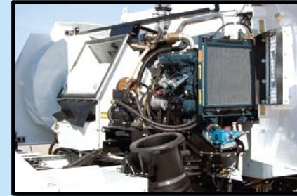
Locking side panels swing away for easy access to the auxiliary engine and blower housing.
